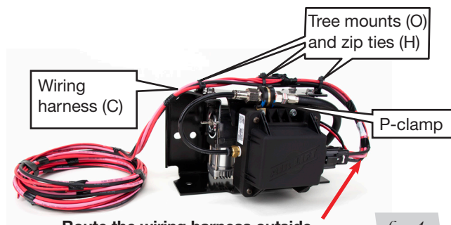
Route the wiring harness outside of the compressor hose.
